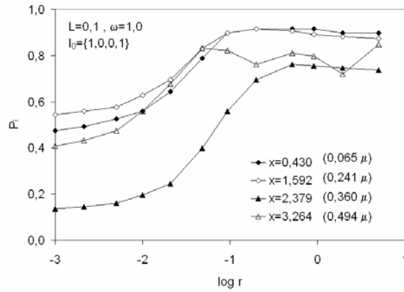
Fig. 13 Computed DOP_L in distance of detector r for a number of size parameters x and optical thickness L = 0.1 mm.
