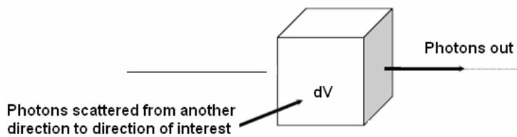
Fig. 6 Increase in the light due to scatter from all directions to the final direction.
