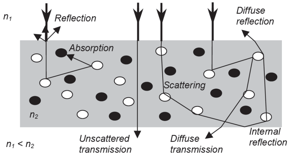
Fig. 2 Schematic diagram for the interaction of light with matter.
