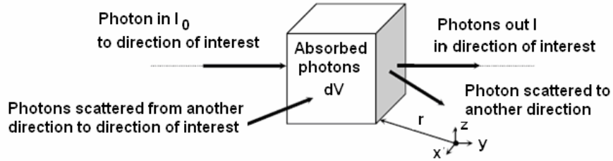
Fig. 3 Model for RTE.
