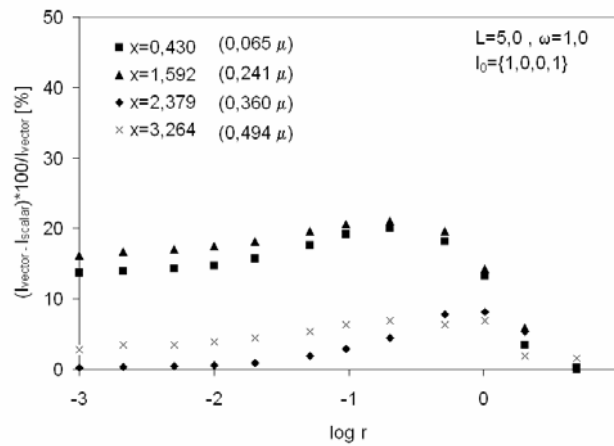
Fig. 12 Difference between the vector and scalar radiative transfer solutions for diffuse light field in distance r for a number of size parameters x and optical thickness L = 5.0 mm.
