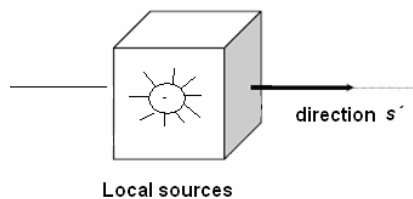
Fig. 7 Local sources of light in material.
