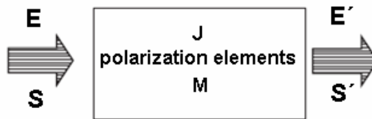
Fig 8 Jones matrices and Mueller calculus.
