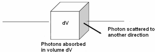
Fig. 5 Attenuation of light due to absorption and scattering.
