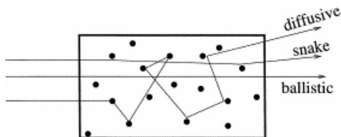
Fig. 1 Trajectories of photons in a random medium.
