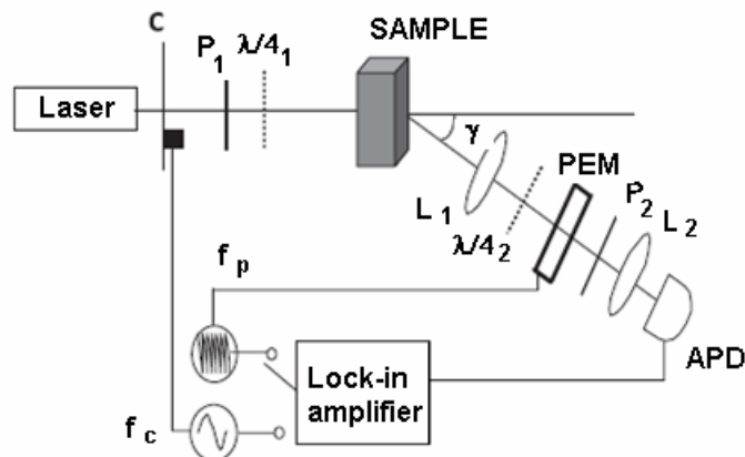
Fig. 10. Scheme of the experimental polarimetry system employing polarization modulation and synchronous lock-in-amplifier detection [19].
